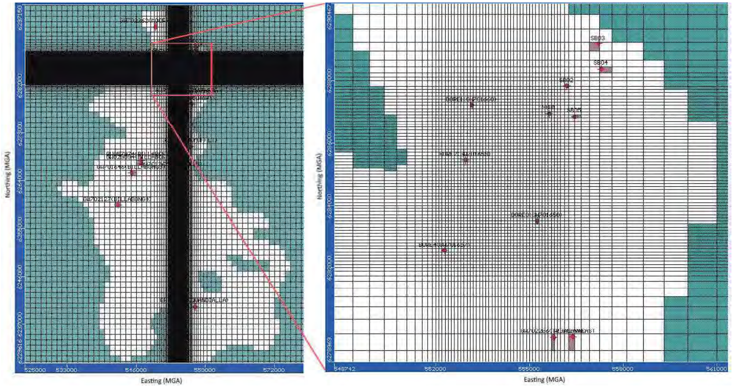
Figure 6-2: Model mesh
