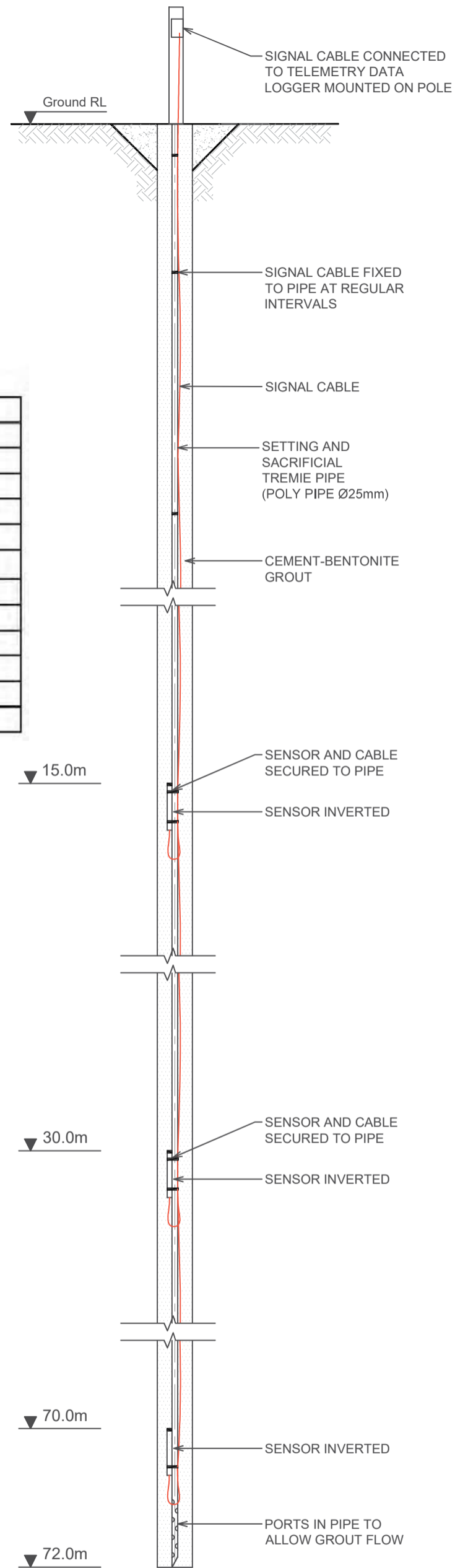
PIEZOMETER SECTION
