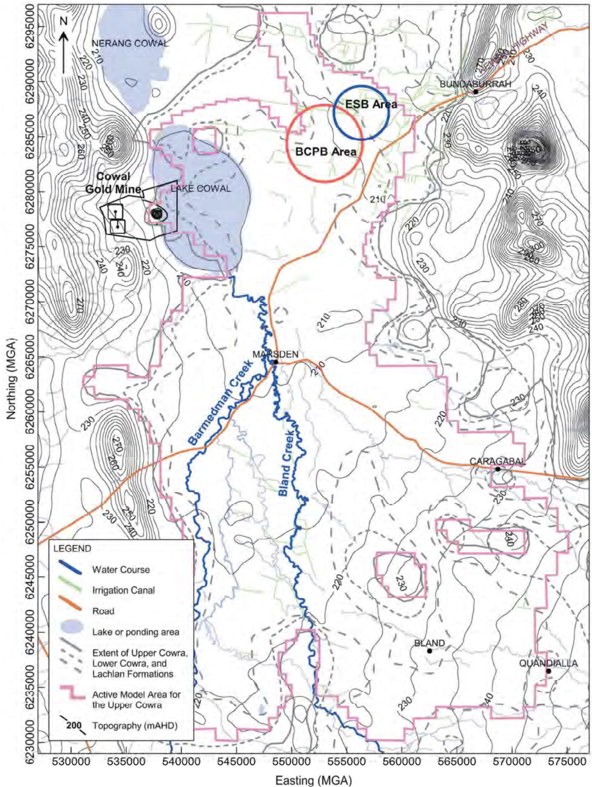
Figure 4-1: Regional topography
