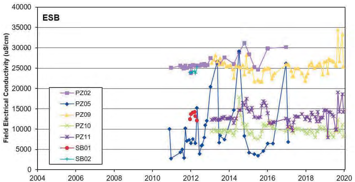
Figure 4-12: Groundwater EC versus time at Evolution monitoring piezometers
