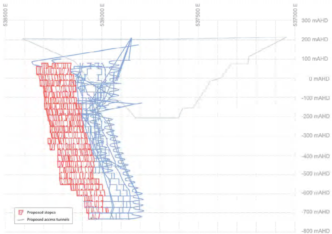
Figure 7-7: Stopes and access tunnels - elevation view looking south (Eastings in m MGA Zone 55)
