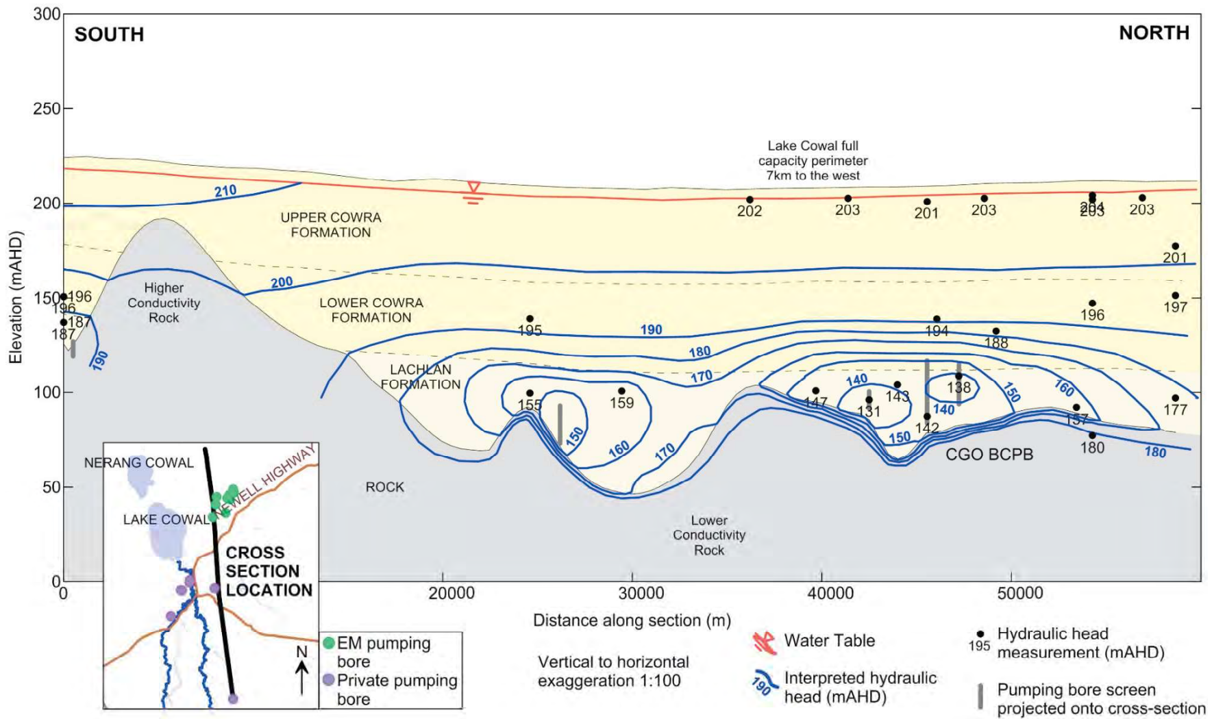
Figure 4-10: Interpreted hydraulic head cross-section for January 2010
