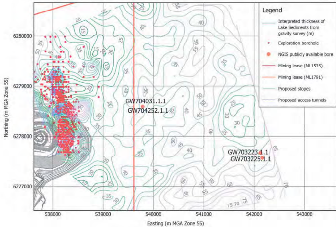
Figure 12: Thickness of the Lake Sediments from gravity survey interpretation
