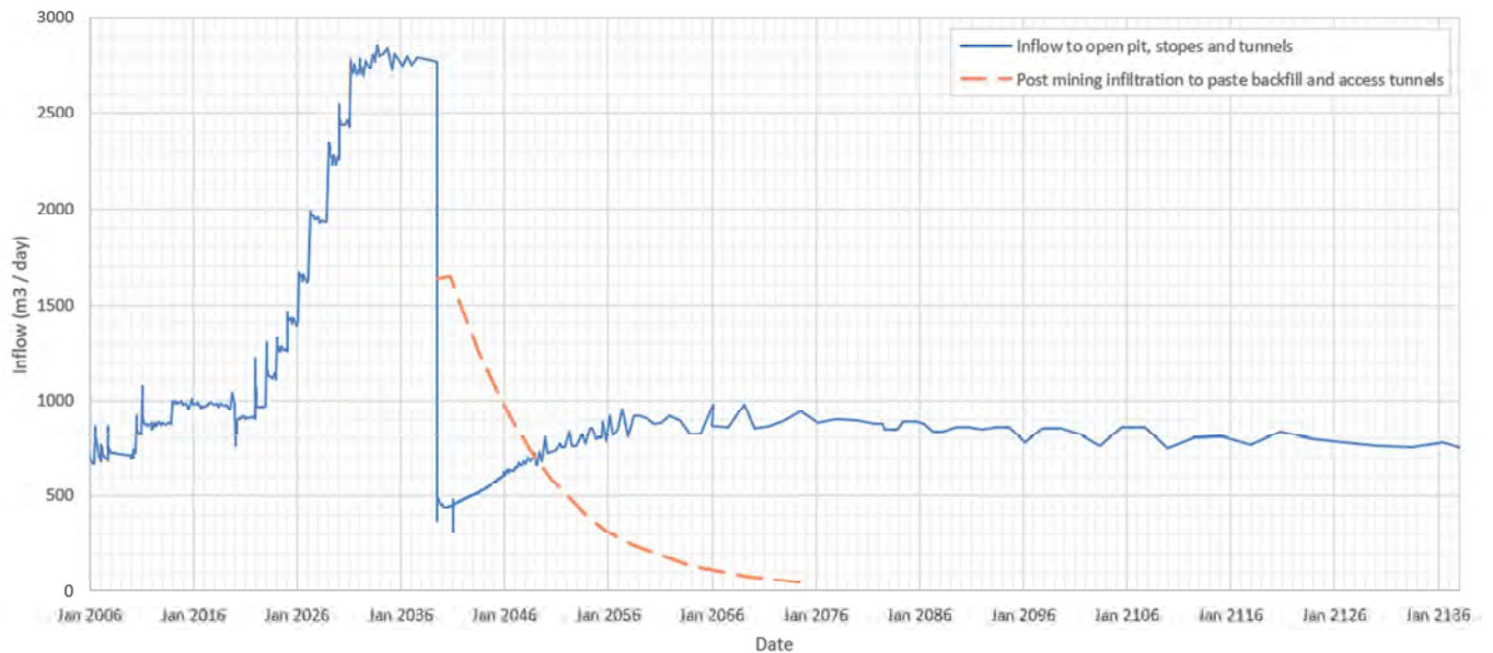
Figure 10-5: Predicted groundwater inflow to the open pit, stopes and access tunnels (2006 to 2138)
