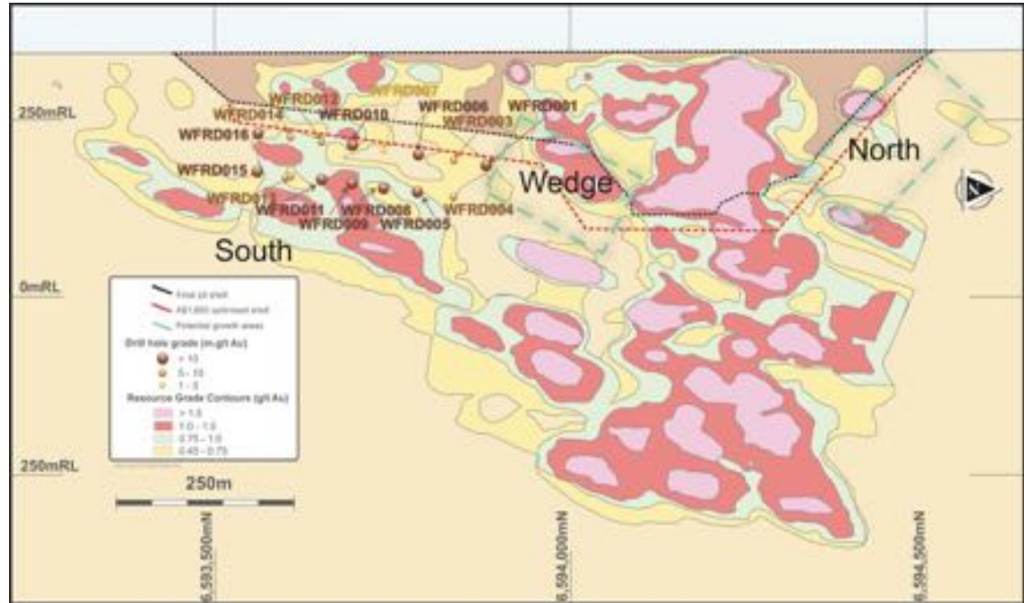
Resource definition drilling showing extensions to mineralisation outside of the current Ore Reserve envelope and future target areas
